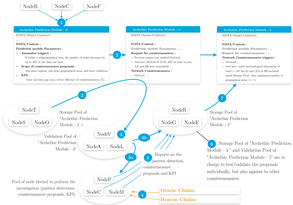
Figure 1.21: Prediction Module
