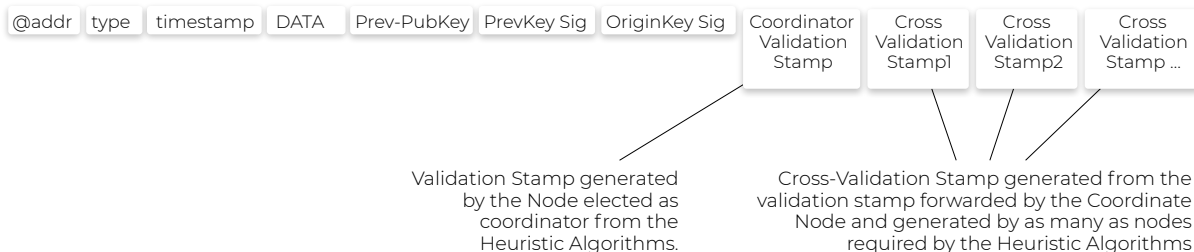
Figure 1.3: Validated Transaction
