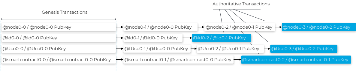
Figure 1.4: Examples of transaction chains
